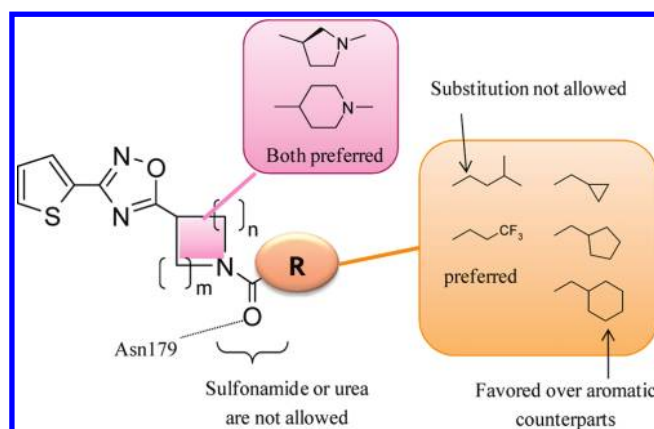
Figure 5. Summary of SAR study with thiofen-2-yl-1,2,4-oxadiazole derivatives.
